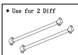
HI903-019 Transverse driver shaft set 2pcs φ 4*87.5mm
