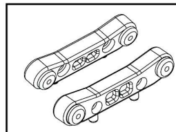
HI903-028 Lower susp. mount block-Fr/Rr
