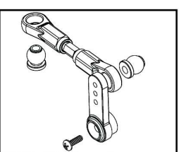
HI903-037 Steering servo horn and linkage 1set
