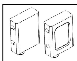
HI903-038 Streering servo mount-A/B
