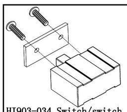
HI903-034 Switch/switch cover/screw
