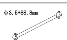
HI903-027 Centre drive shaft-Fr φ 3.5*88.8mm
