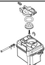
HI903-057 Fuel tank unit
