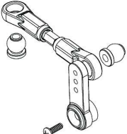
HI903-037 Steering servo horn and linkage 1set
