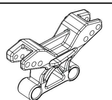
HI903-005 Shock tower
