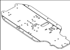
HI903-042 Chassis (AL6061T) 1pcs
